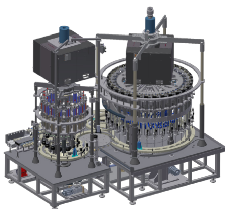
Flexible filling and closing machine from Tölke for handling up to 300 bottles/min at a fill volume of up to 250 ml. (Rendering: Tölke)
