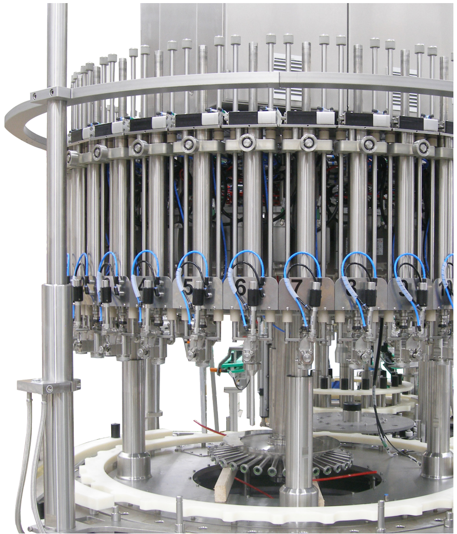
The monoblock system has space for 36 filling stations, in which each filling needle is driven by a LinMot linear motor. This allows rapid product changeover and broadens the range of application of the filling and closing machine. (Photo: Rossmann)
